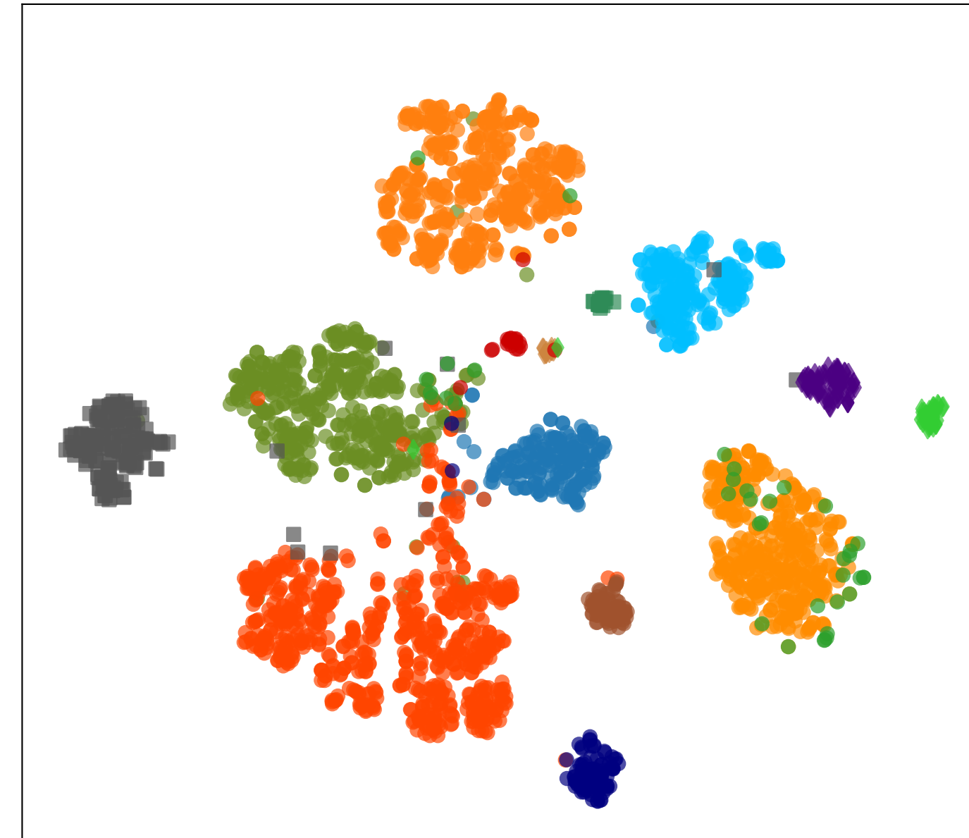
Pred Classes
