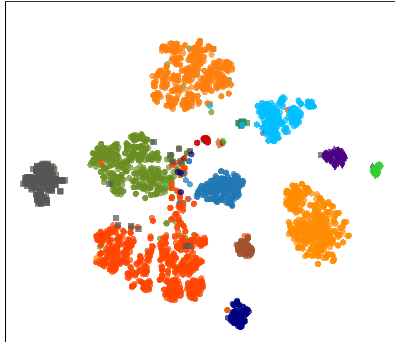
True Classes
