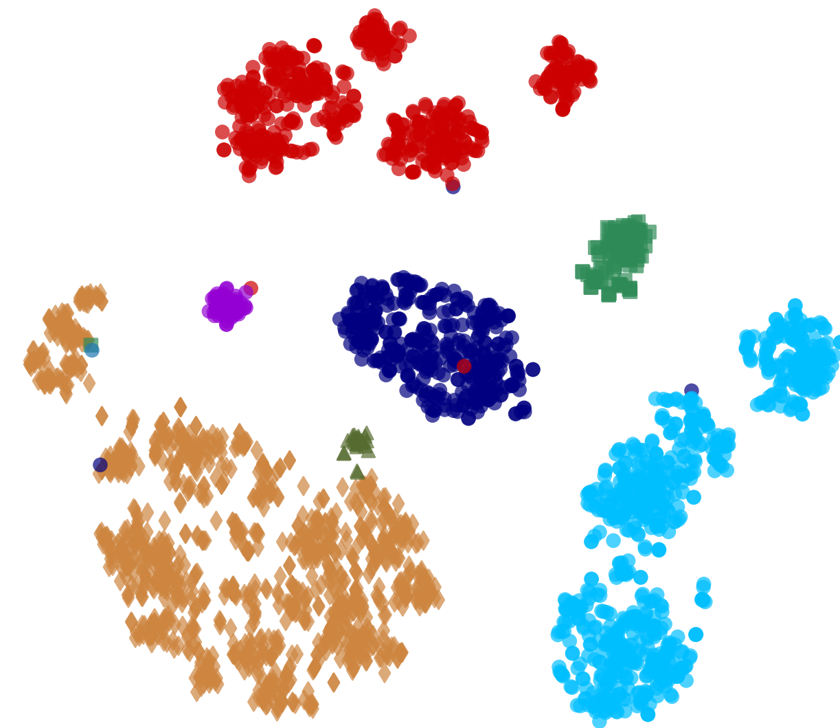
Pred Classes
