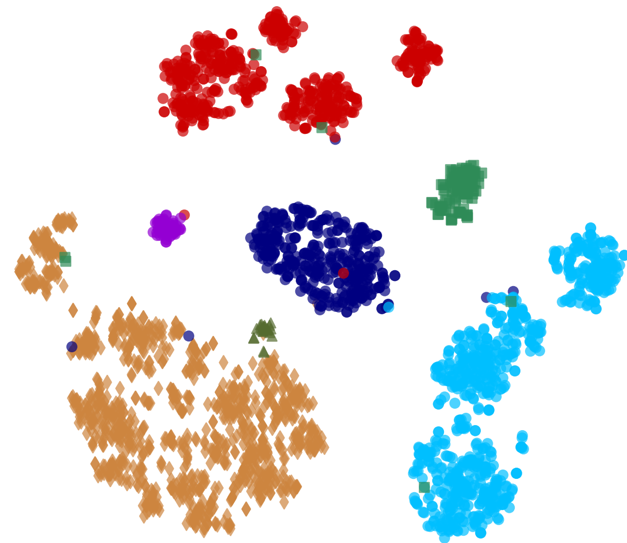
True Classes
