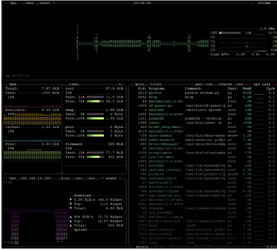
Figure 17: HOG - Idle state (No face)
