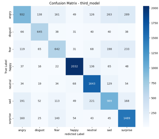
Figure 16: Confusion Matrix - third_model
