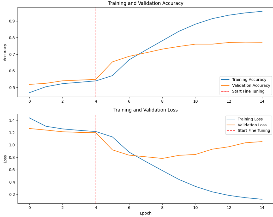
Figure 9: Training and validation metrics for the ResNet101 second run. The deeper architecture benefits significantly from the two-stage fine-tuning approach.
