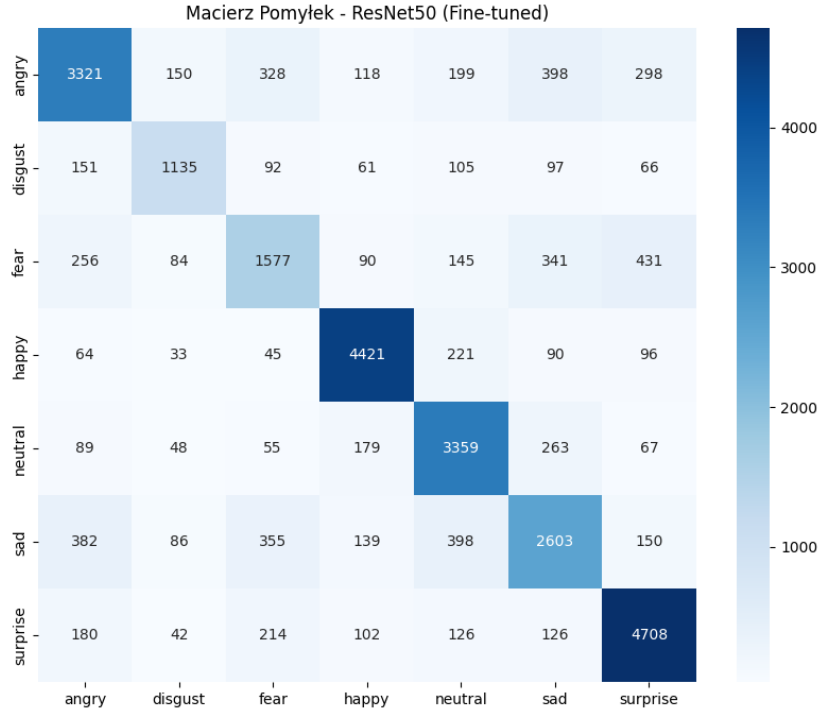
Figure 6: Confusion matrix for the optimized ResNet50 model.
