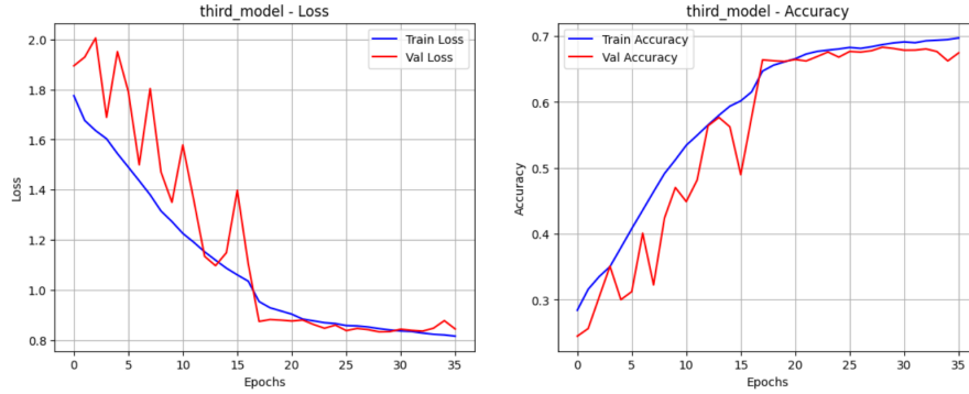
Figure 19: Graph of validation and training loss/accuracy for third_model
