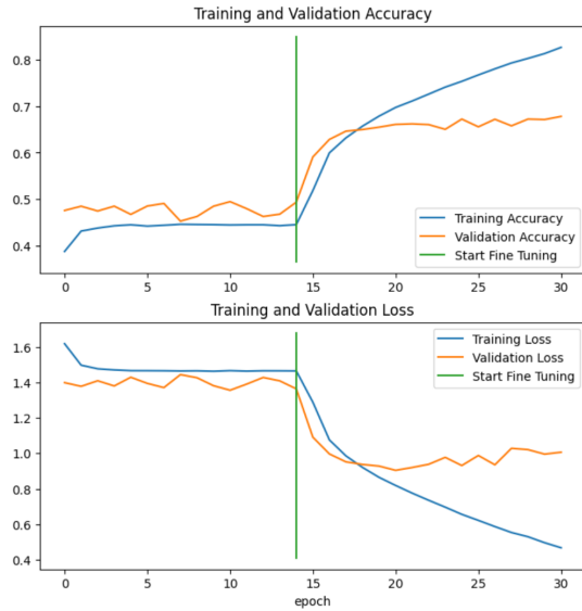
Figure 23: Fine-Tuning progress for ResNet50
