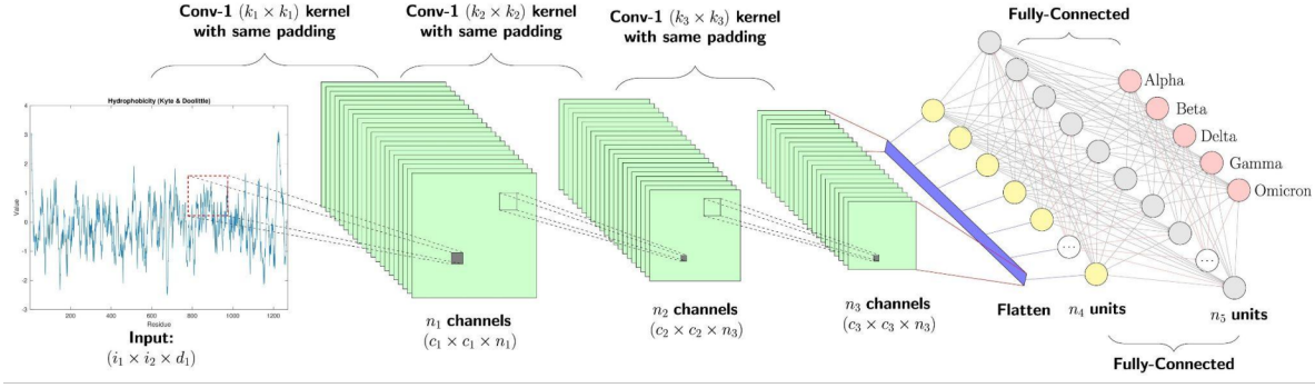
Figure 14: CNN network example
