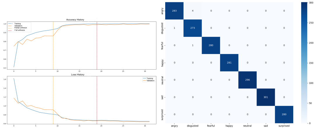
Figure 11: Metrics for Dataset 1 Evidence of extreme overfitting to specific prompts.
