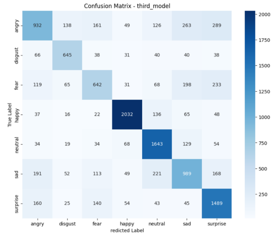
Figure 18: Confusion Matrix - third_model
