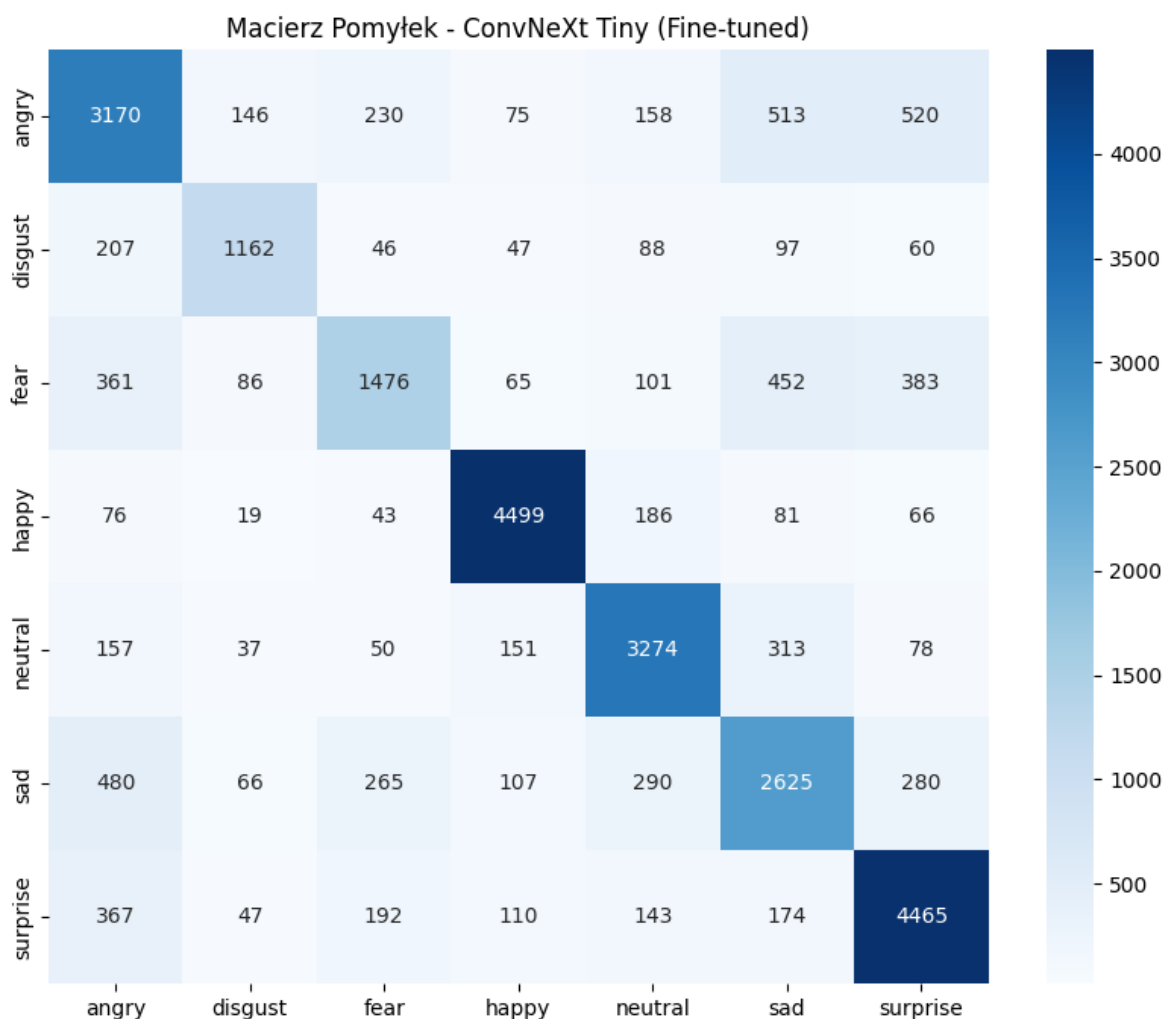
Figure 24: Confusion Matrix - ConvNeXt Tiny (Fine-tuned, 10 epochs)
