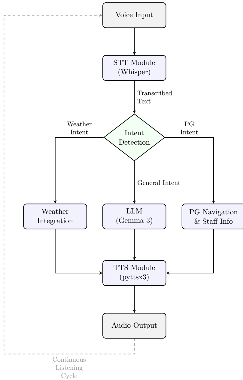
Figure 31: NLP Pipeline Data Flow.
