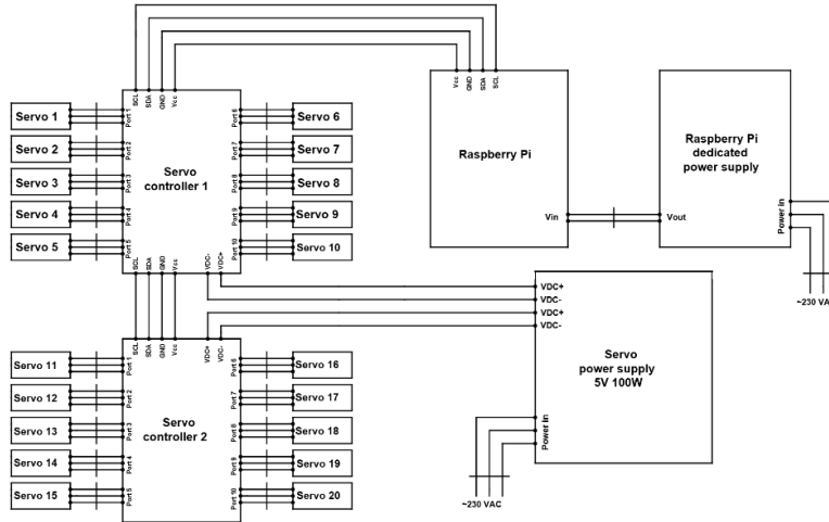
Figure 2: Electrical wiring diagram
