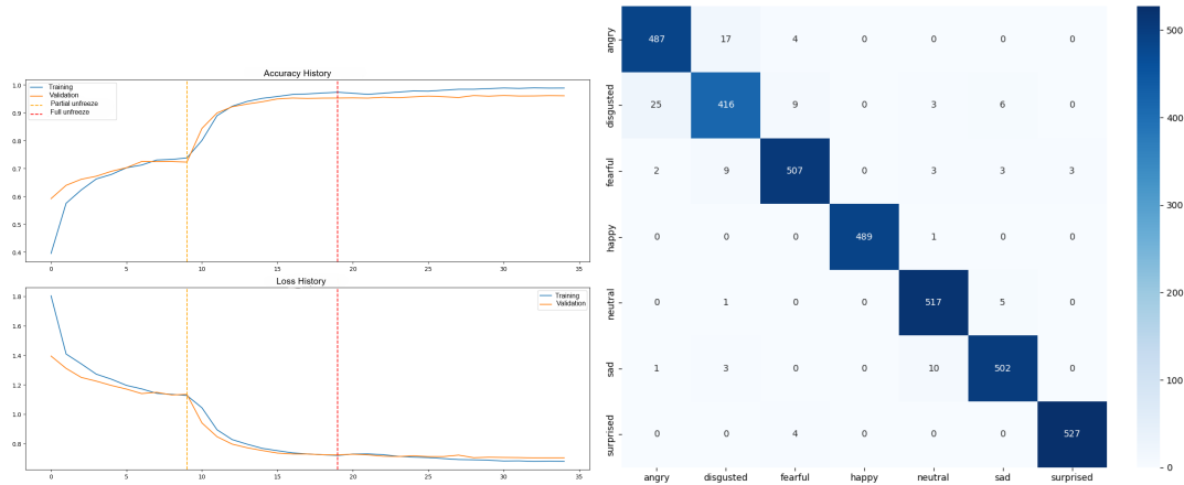
Figure 13: Metrics for Dataset 3 High validation scores masking poor practical utility.
