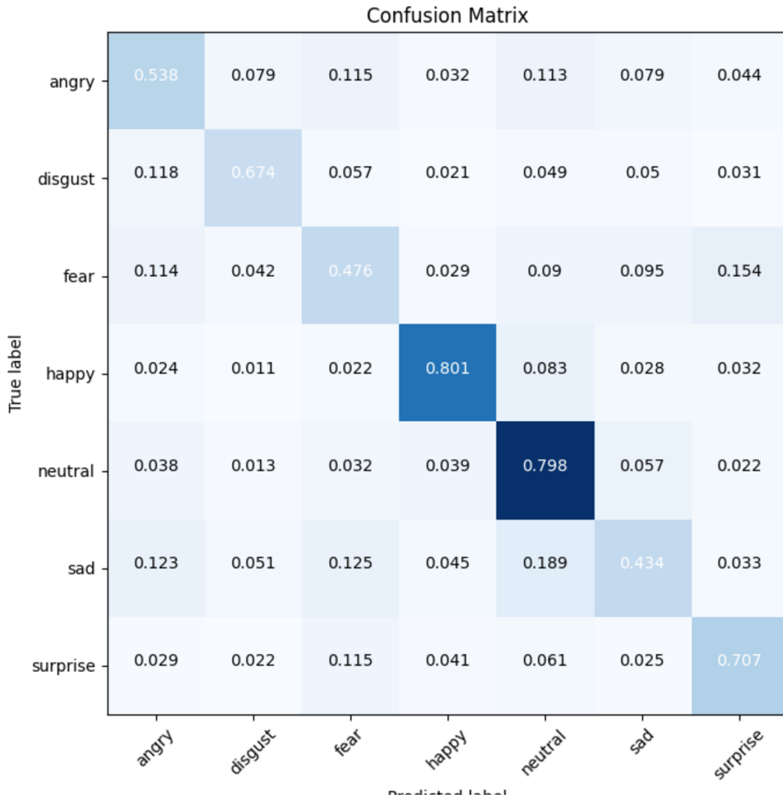
Figure 15: Confusion matrix
