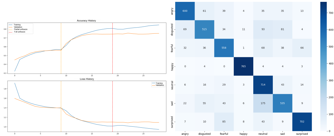
Figure 12: Metrics for Dataset 2 Balanced training with realistic generalization.
