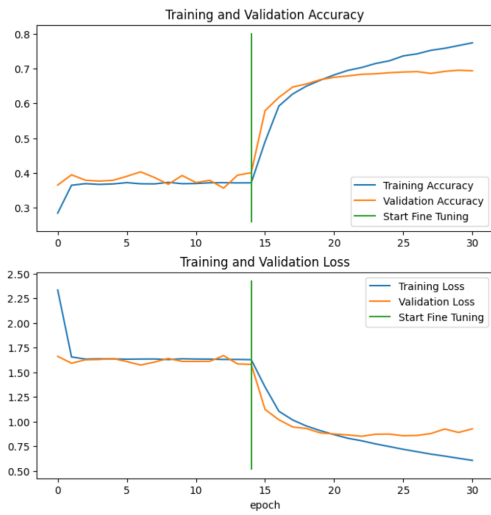
Figure 22: Fine-Tuning progress for VGG19
