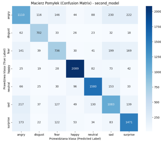
Figure 17: Confusion Matrix - second_model
