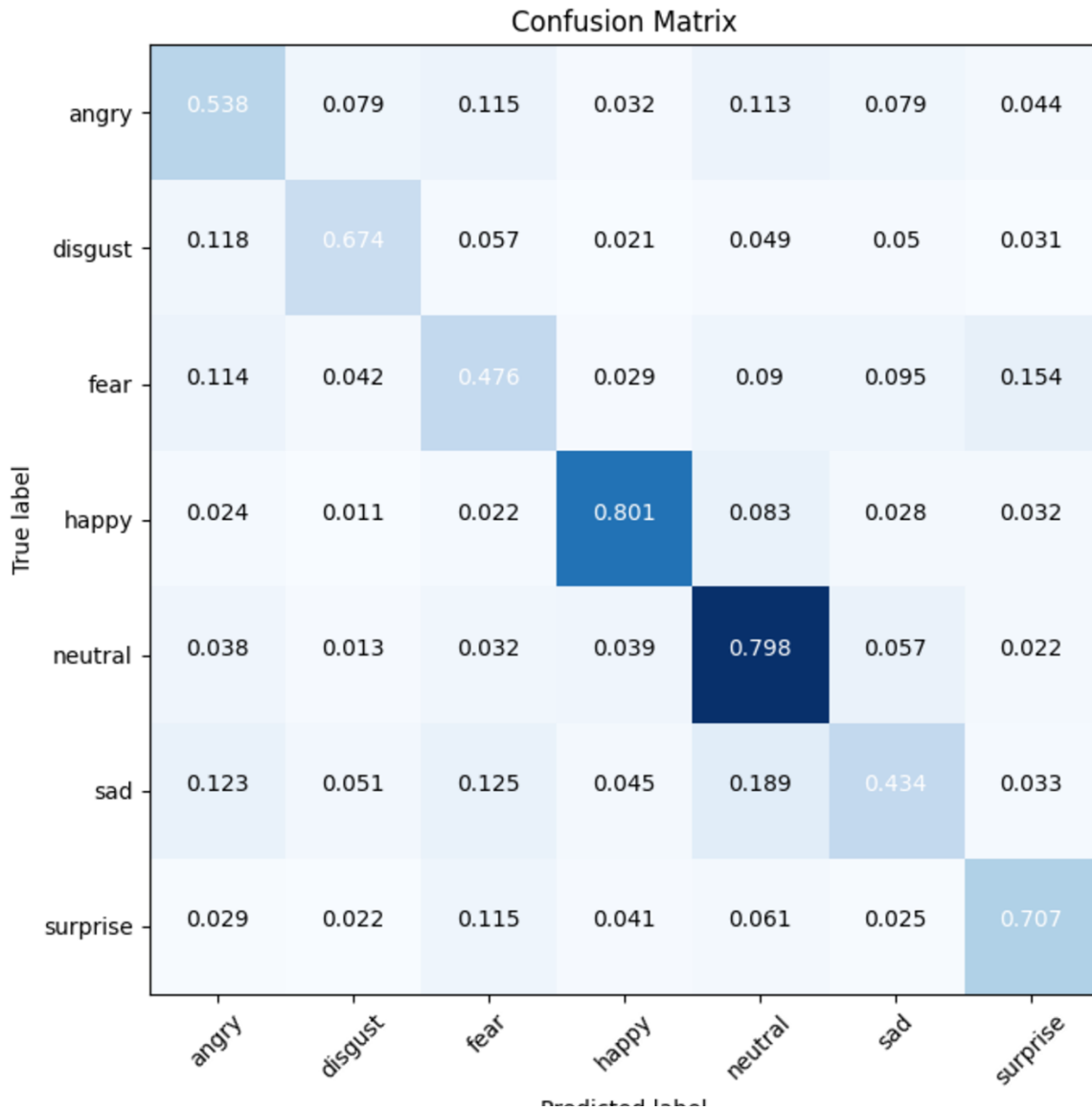
Figure 13: Confusion matrix
