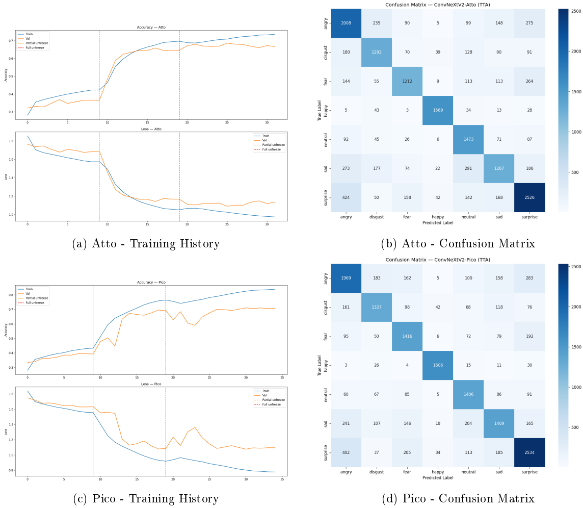
Figure 13: Comparison of training histories and confusion matrices for the ConvNeXtV2 Atto and Pico models.
