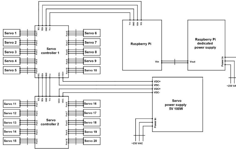
Figure 2: Electrical wiring diagram
