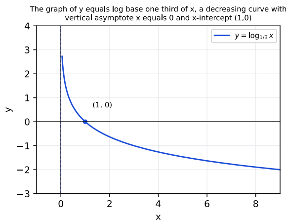
Figure 2: The graph of y equals log base one third of x , a decreasing curve with vertical asymptote x equals 0 and x -intercept (1, 0)
