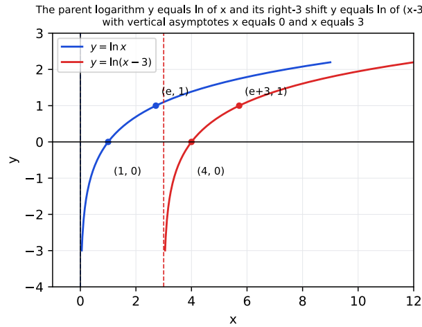
Figure 4: The parent logarithm y equals \ln of x and its right-3 shift y equals \ln of (x-3) , with vertical asymptotes x equals 0 and x equals 3
