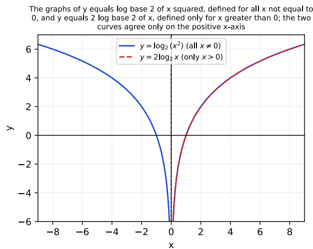
Figure 5: The graphs of y equals log base 2 of x squared, defined for all x not equal to 0, and y equals 2 log base 2 of x , defined only for x greater than 0; the two curves agree only on the positive x -axis
