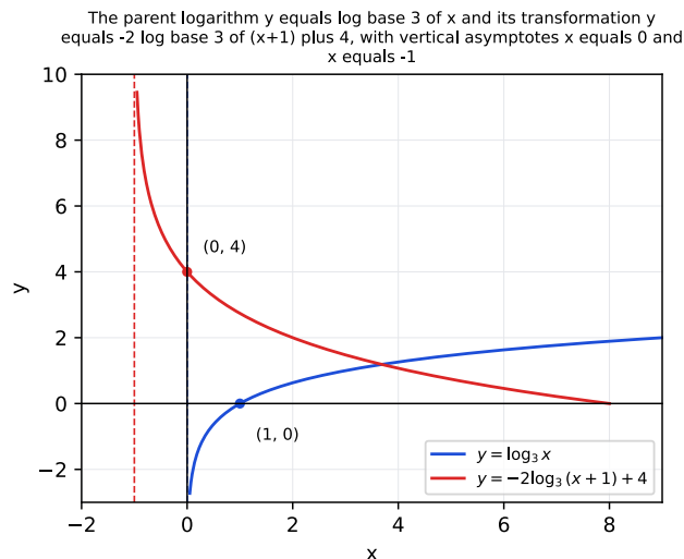
Figure 3: The parent logarithm y equals log base 3 of x and its transformation y equals -2 \log base 3 of (x+1) plus 4, with vertical asymptotes x equals 0 and x equals -1
