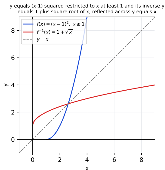
Figure 1: The graph of y equals (x-1) squared restricted to x at least 1 and its inverse y equals 1 plus square root of x , reflected across y equals x
