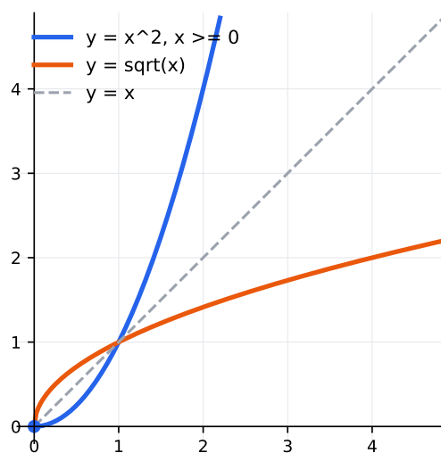
Figure 3: y equals x squared for x at least 0 and its inverse, the square root function
