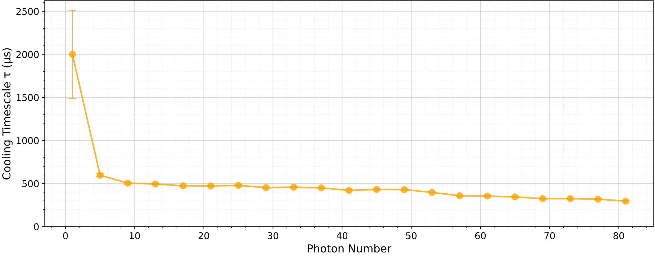
Effect of Photon Number on Cooling Timescale
