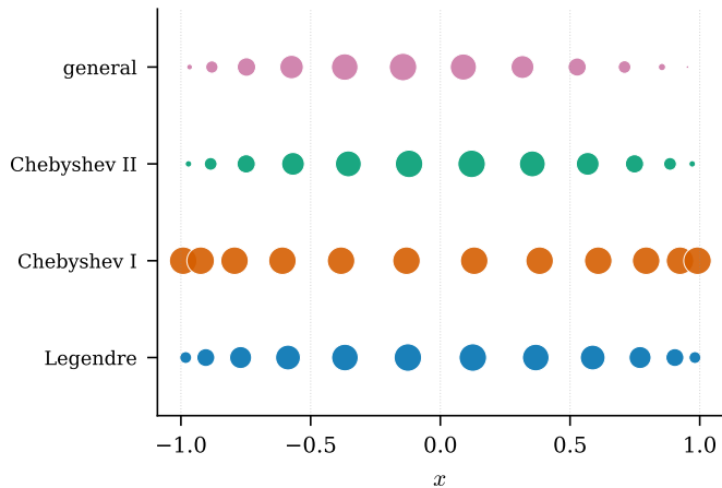
(b) n = 12 Gauss-Jacobi nodes
