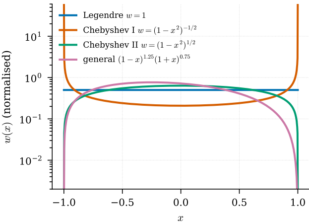
(a) The weight defines L_w^2([-1, 1])
