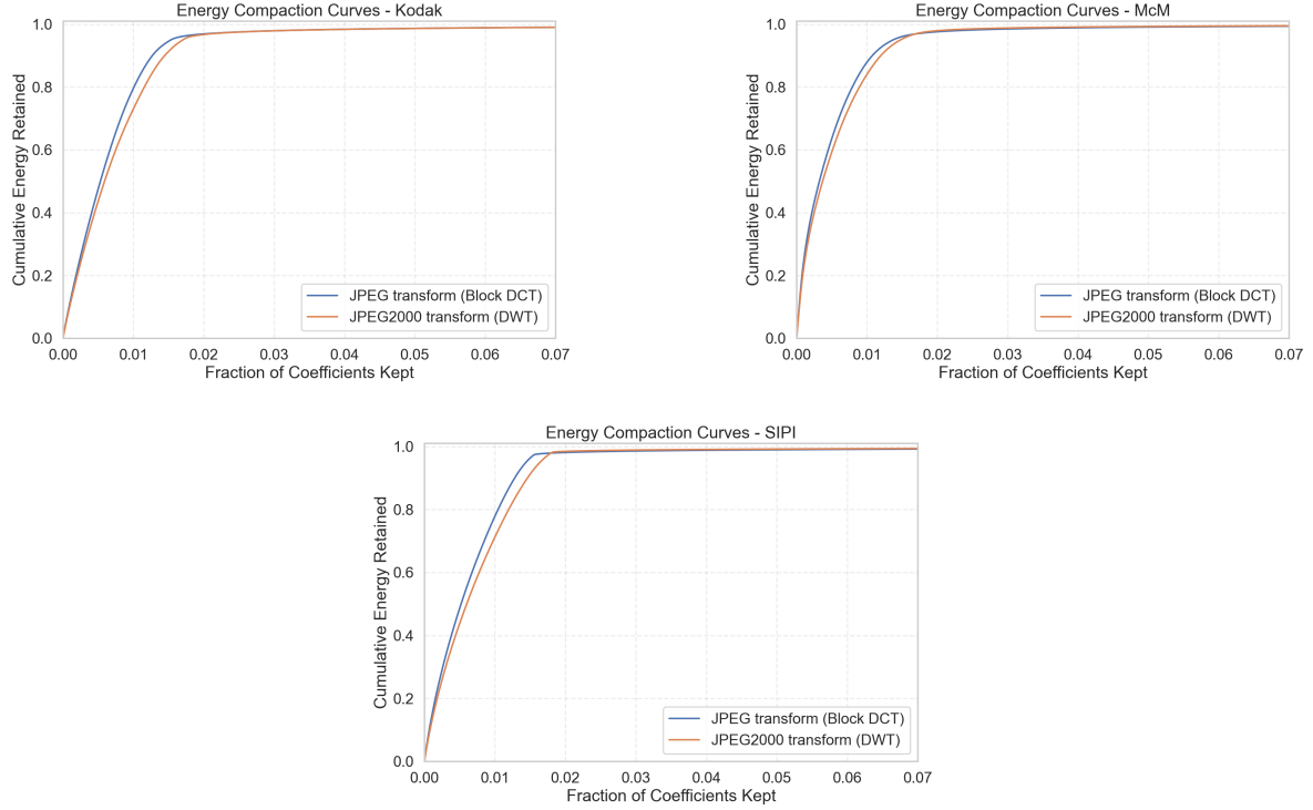
Figure 4: Energy compaction curves for transform coding on representative images from each dataset.
