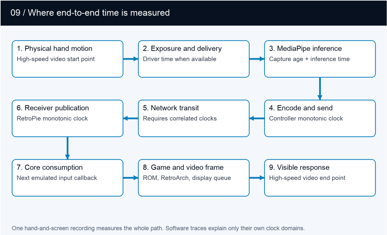
End-to-end latency boundaries from the physical hand and camera through MediaPipe, RetroPie, the emulator, and the visible game
