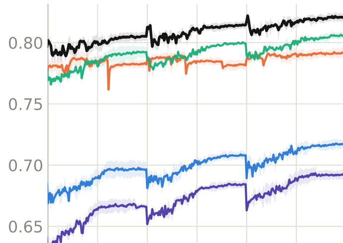
Sparsity 0.95
