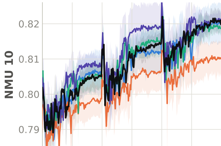
Sparsity 0.1
