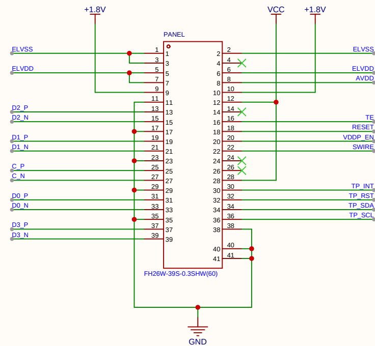
DXQ Panel 5.48" Connector
