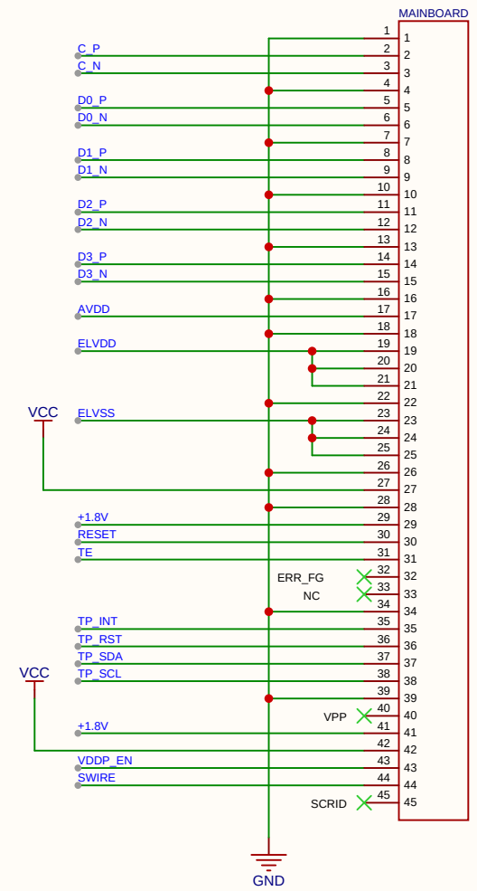
piBrick Mainboard
