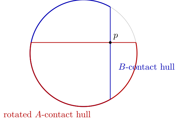
FIGURE 1. In the doubled-angle circle, a gap in each proper contact set creates an exposed chord. One chord can be rotated so that the two relative interiors cross. The crossing point belongs to both contact hulls but not to the hull of the common contact directions.
