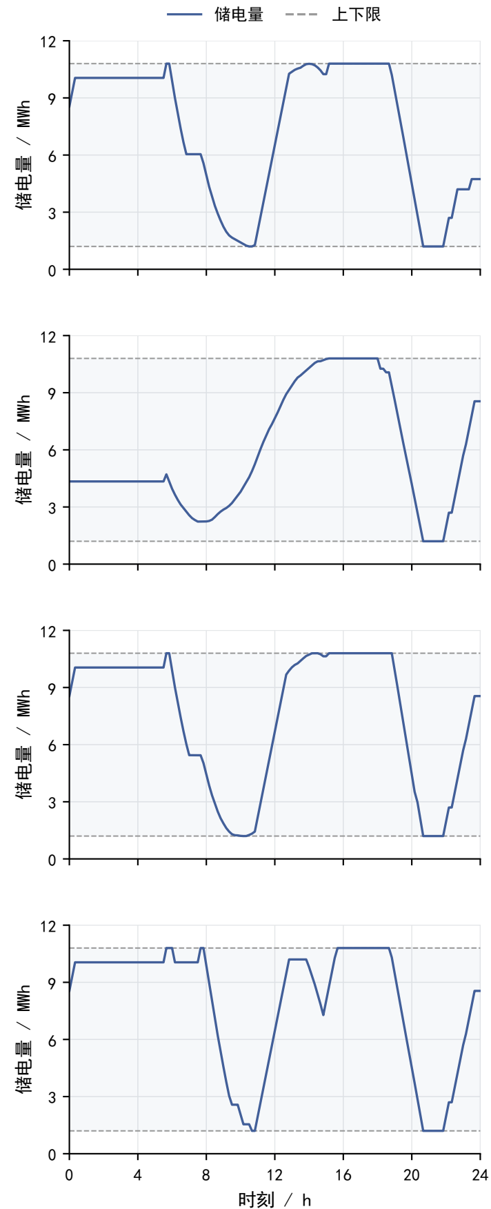
(c) 电池储电量及运行范围
