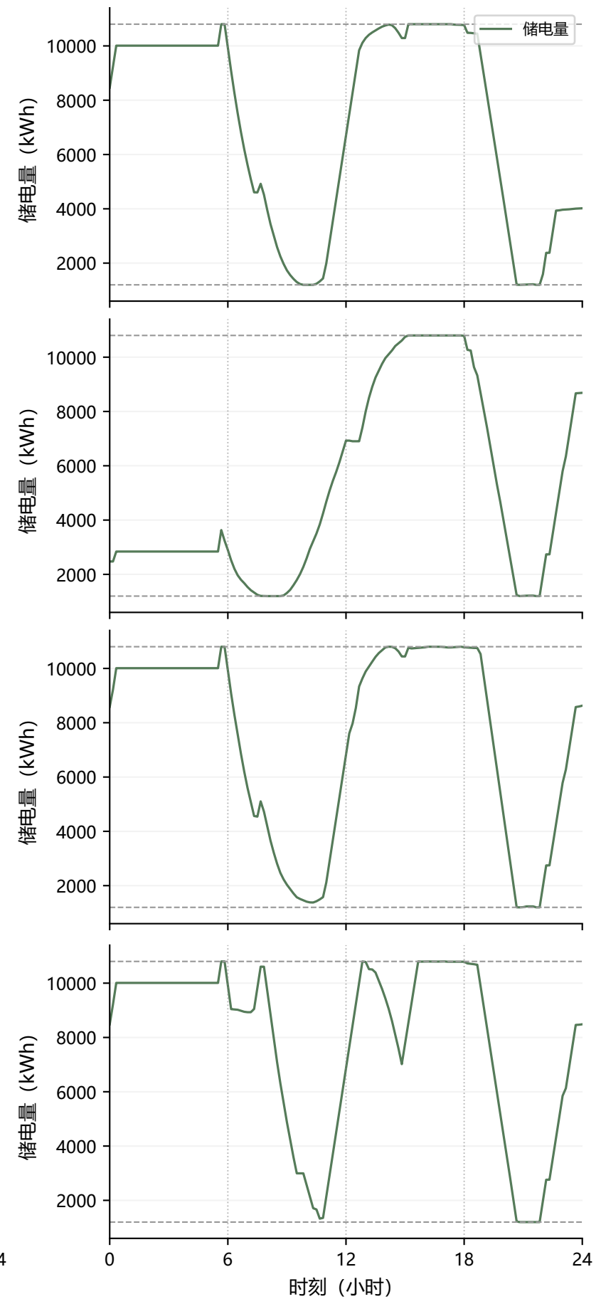
跨时段储能衔接
