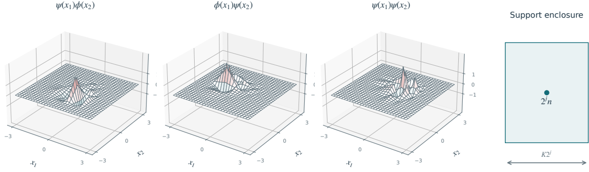
Figure 4.18. 2-D wavelets and a schematic support centered at (2^j n_1, 2^j n_2) , with width K2^j (right).
