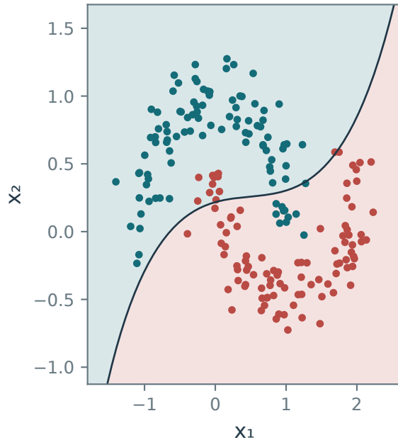
Gaussian kernel \sigma = 1.5
