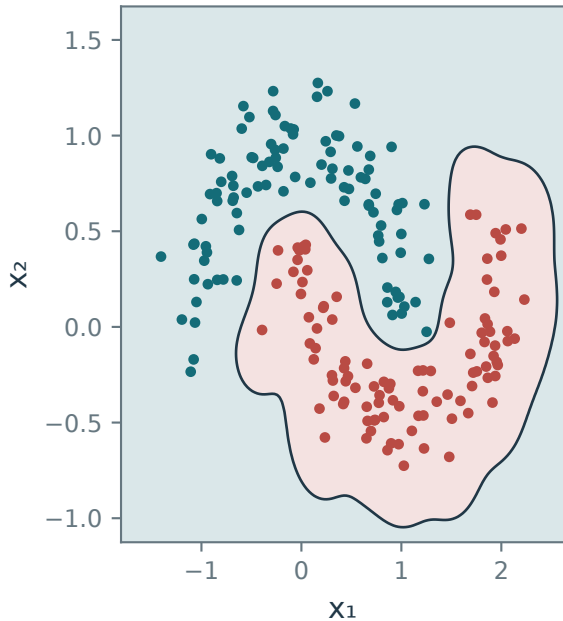
Gaussian kernel \sigma = 0.15
