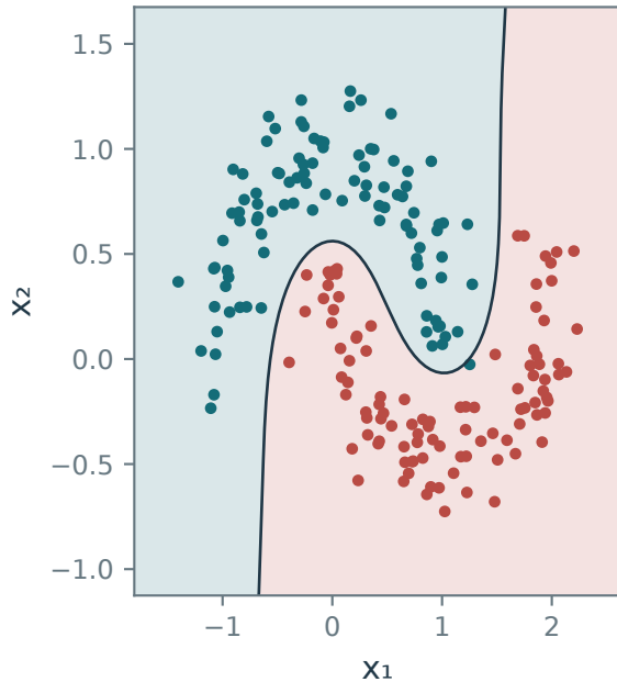
Gaussian kernel \sigma = 0.5
