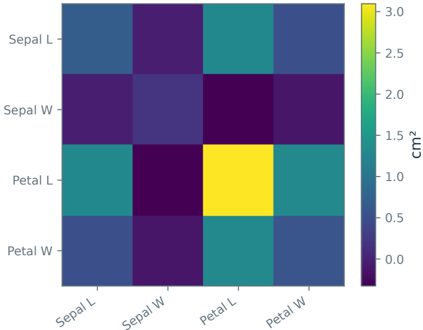
Empirical covariance (Iris)
