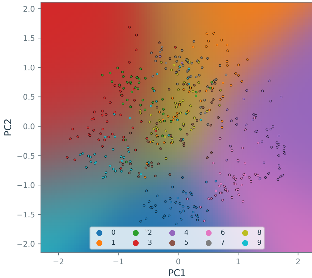
Mixture of all ten class colors
