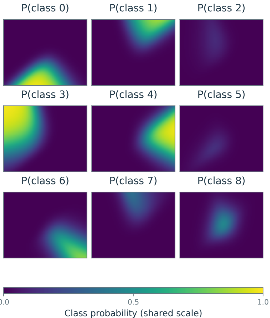
Probabilities on the affine two-PC slice through the training mean
