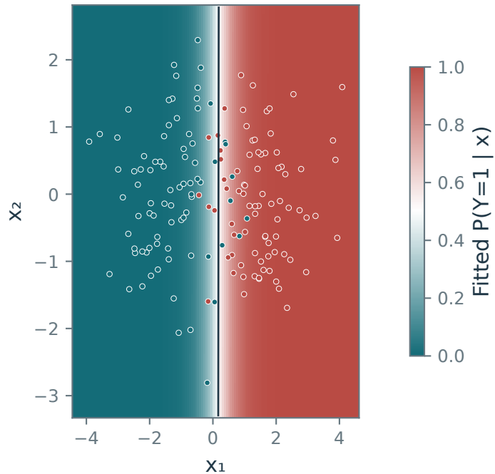
Mean separation 3
