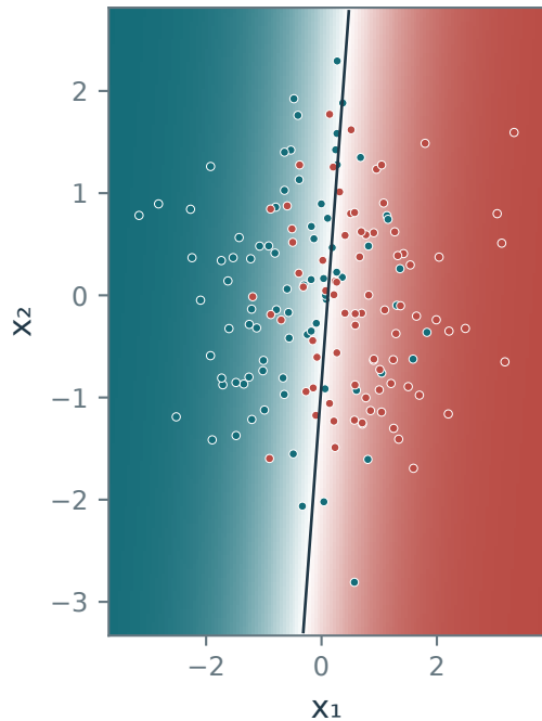
Mean separation 1.5
