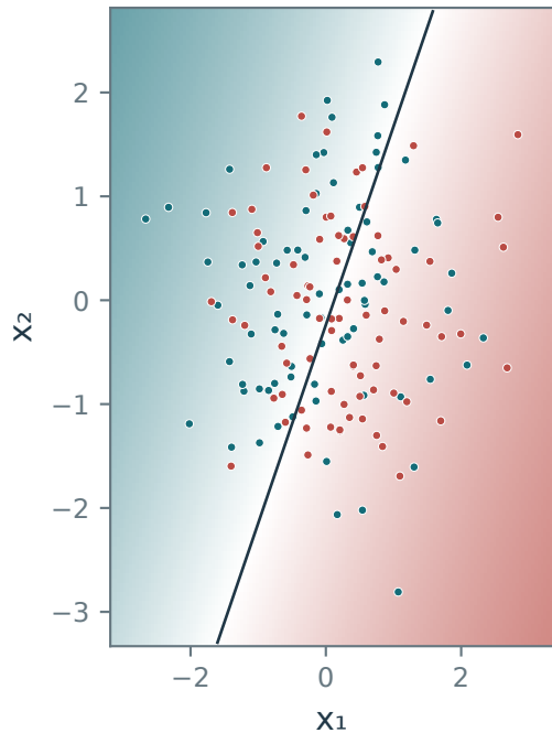
Mean separation 0.5
