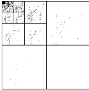
Wavelet support
