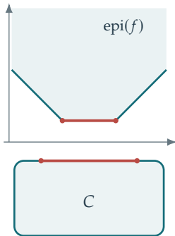
Convex, not strictly convex
