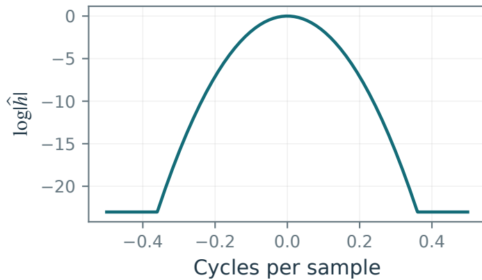
Gaussian kernel spectrum
