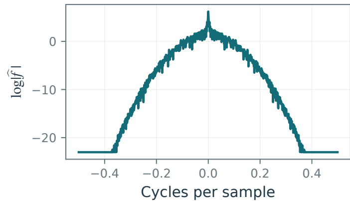
Filtered signal spectrum
