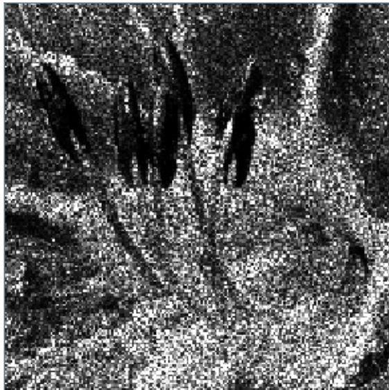
Gamma speckle model
