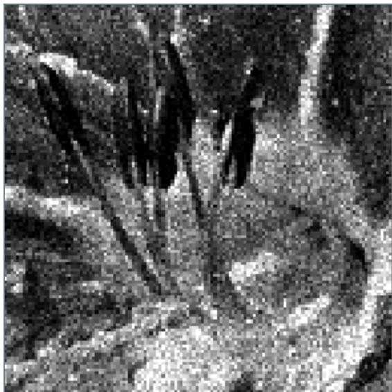
Noisy: 11.9 dB
