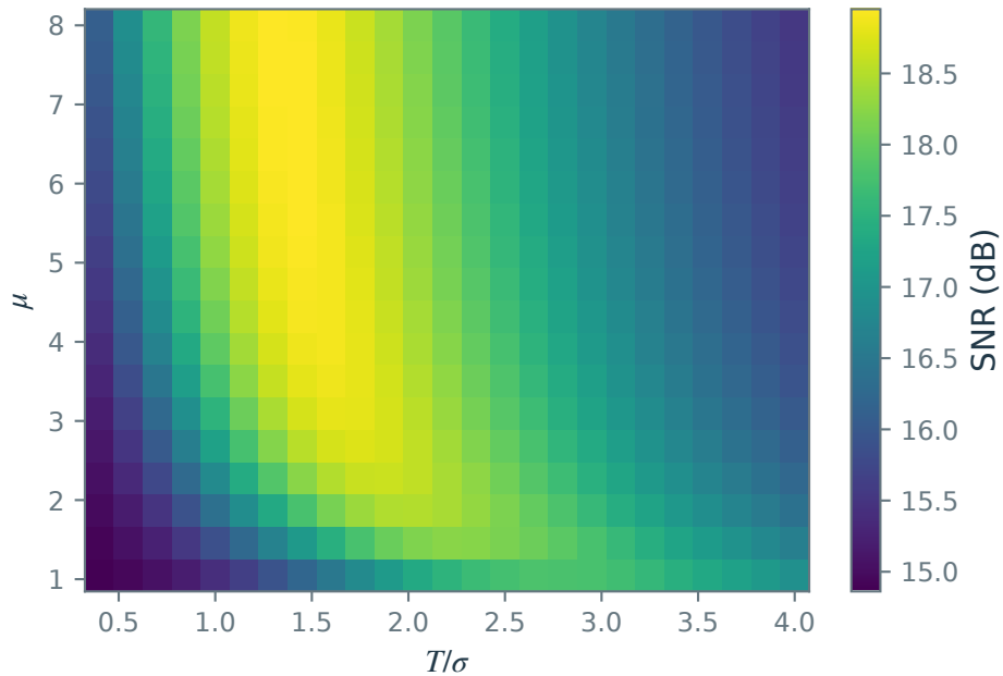
Measured reconstruction SNR
