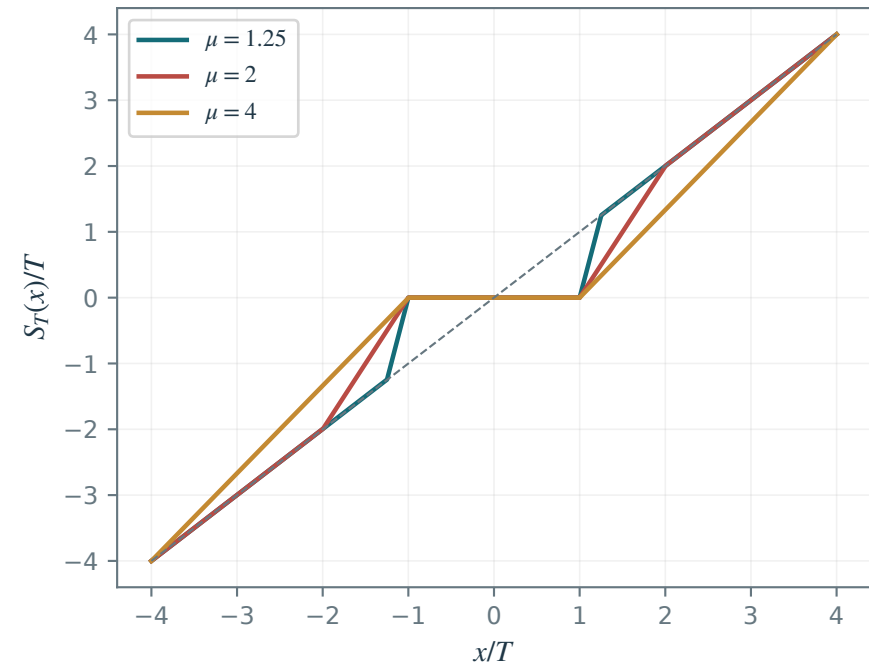
Semi-soft thresholding
