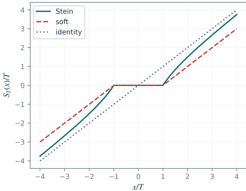
Stein thresholding
