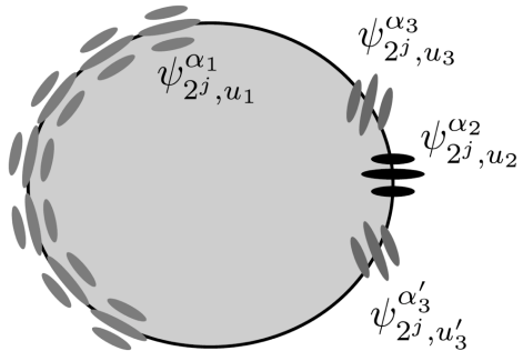
Directional wavelets
