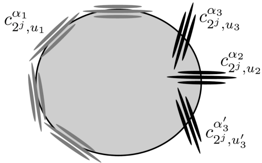
Curvelets
