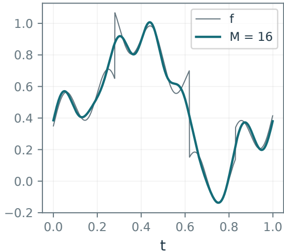
Low-frequency Fourier: M = 16
