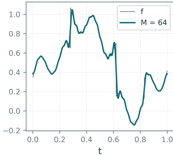
Low-frequency Fourier: M = 64
