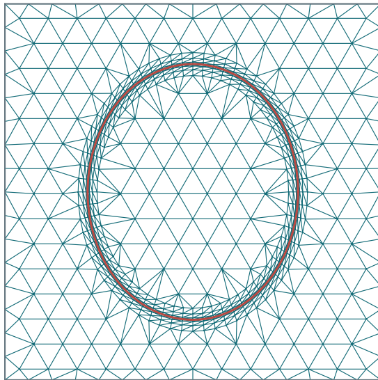
Thin triangles along the boundary
