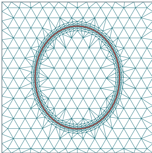
1390 contour-aligned triangles
