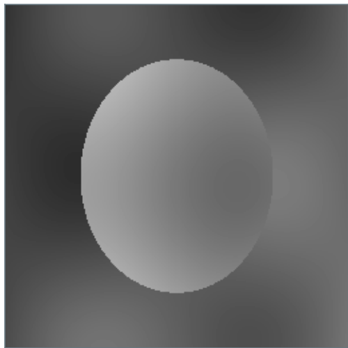
Smooth piecewise cartoon
