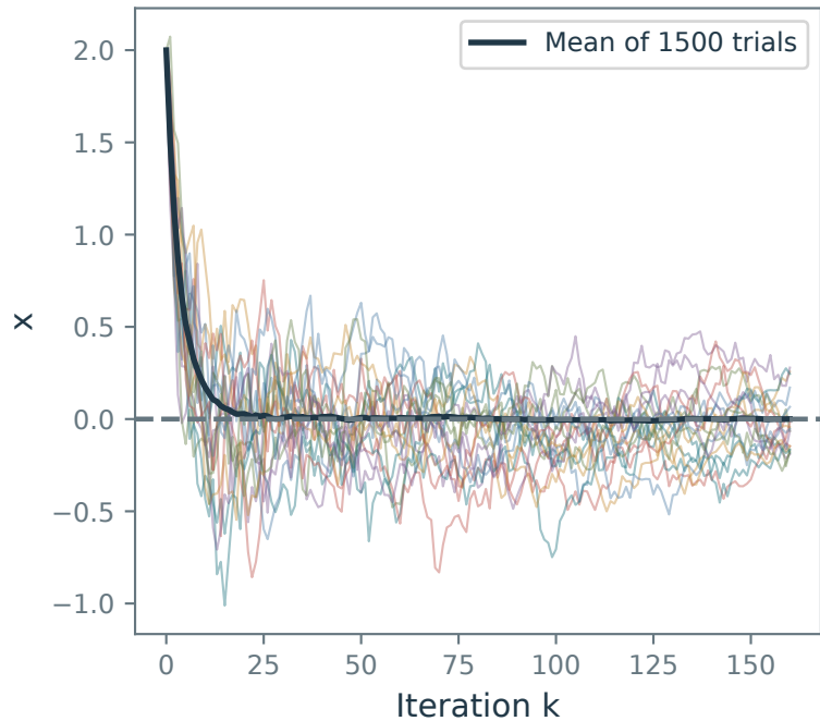
Independent stochastic trajectories
