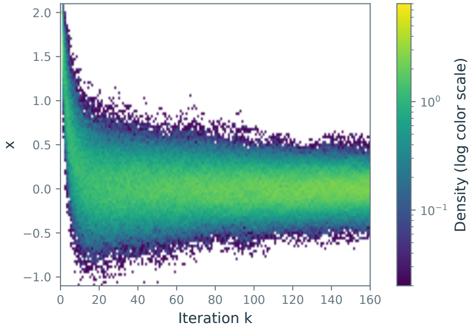
Empirical distribution of iterates
