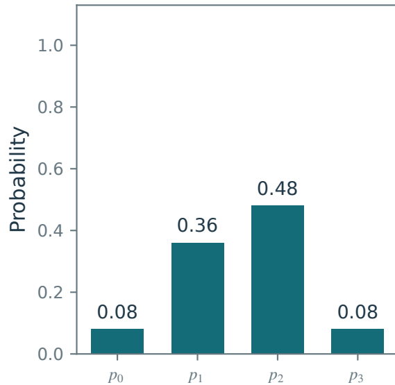
H(p) = 1.62 bits
