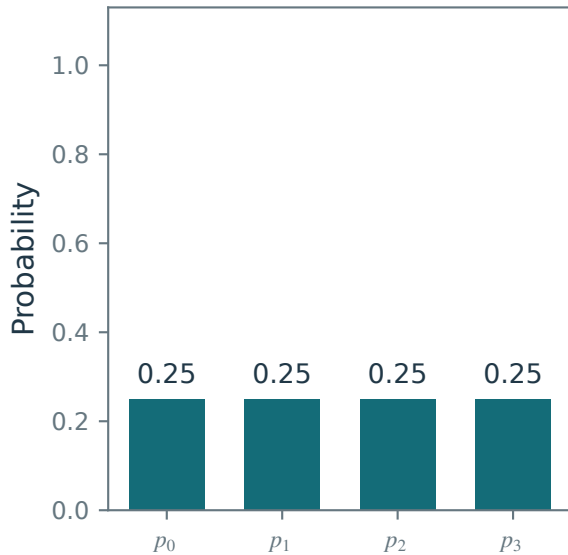
H(p) = 2 bits
