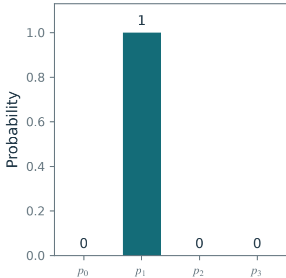
H(p) = -0 bits
