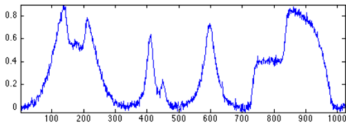
Observation y = h \star f_0 + w
