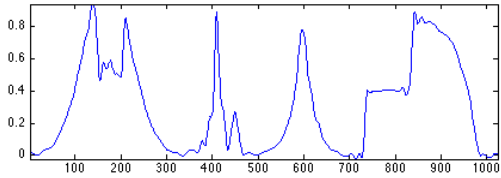
\ell^1 recovery f^\star
