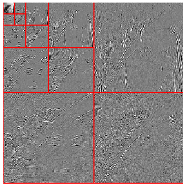
Coefficients \langle f, \psi_m \rangle
