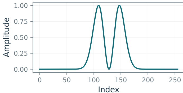
Discrete pseudoinverse (note vertical scale)
