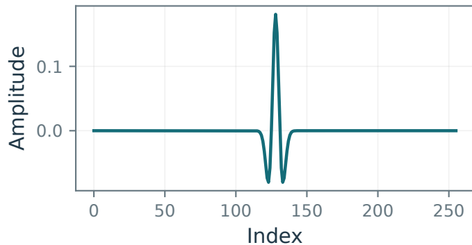
Transmitted second-Gaussian-derivative pulse
