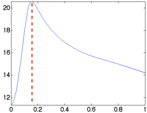
TV regularization
