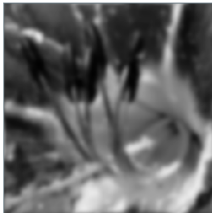
Heat: t = 4
