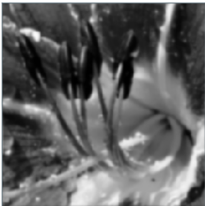
Heat: t = 1
