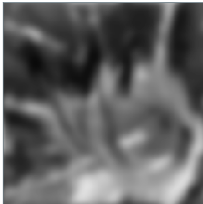
Heat: t = 16
