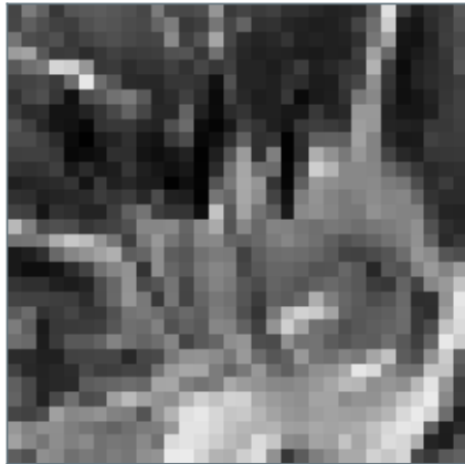
j = -5: 32 \times 32
