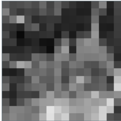
j = -4: 16 \times 16
