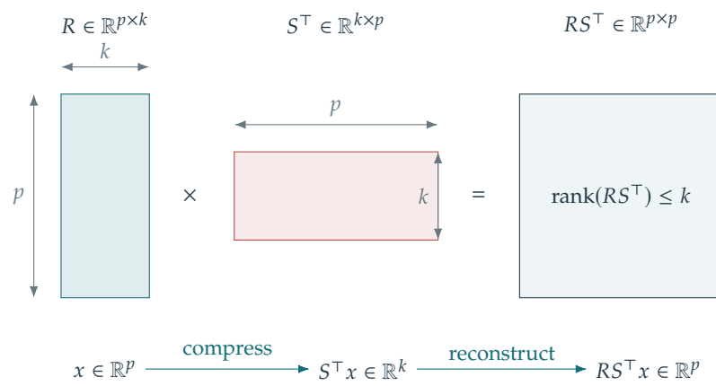
Figure 13.5. Linear compression followed by reconstruction.
