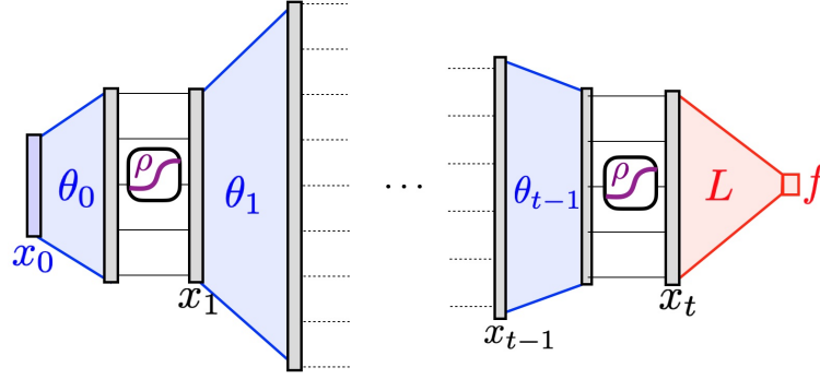
Figure 15.13. Multilayer-perceptron parameterization.
