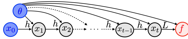
Figure 15.14. Computational graph for a recurrent architecture.
