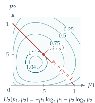
Entropy in the positive quadrant
