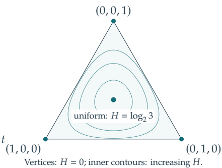
Three-symbol simplex
