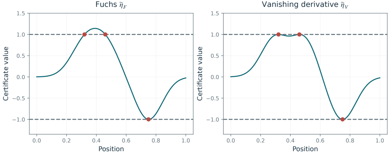
Figure 11.11. Continuous representations of the precertificates \eta_F and \eta_V for a convolution operator A .
