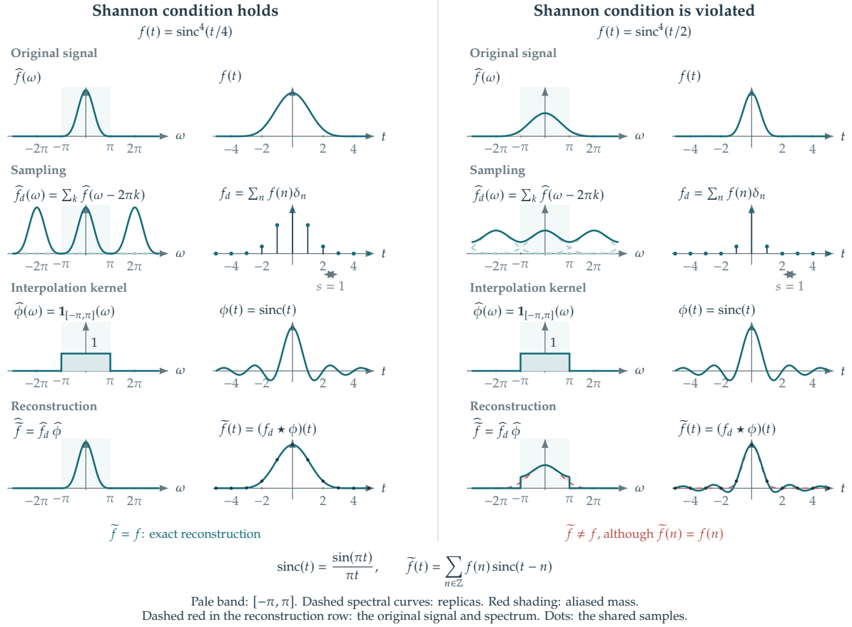
Figure 1.4. Sampling and Shannon interpolation in the frequency and time domains, with unit sample spacing. Left: the bandlimiting condition of Theorem 1.2 holds. Right: overlapping spectral replicas cause aliasing; the reconstructed signal still passes through every sample. The rows show the original signal, sampling, the interpolation kernel, and reconstruction.
