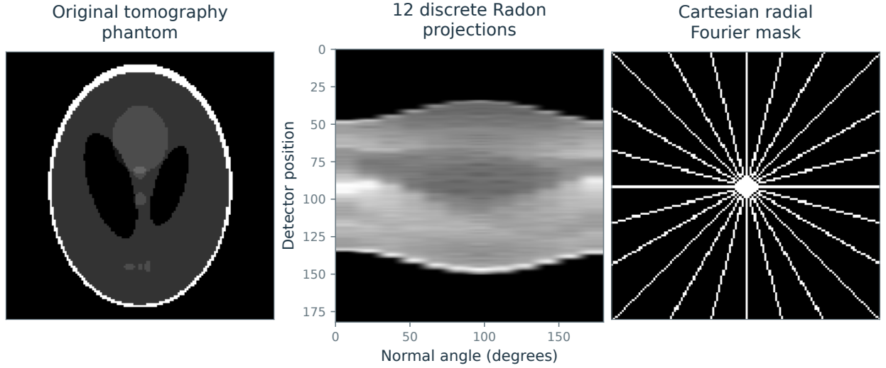
Figure 9.8. Tomography test phantom, discrete Radon projections, and a Cartesian radial Fourier-sampling mask.
