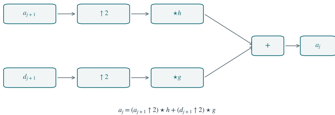
Figure 4.15. Inverse filter-bank reconstruction.
