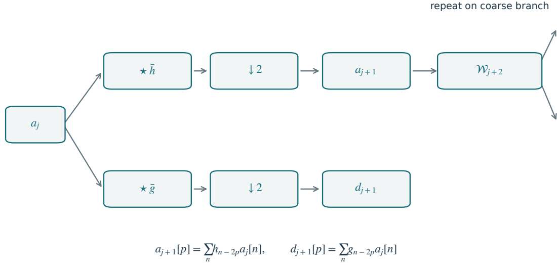
Figure 4.10. Forward filter bank decomposition.
