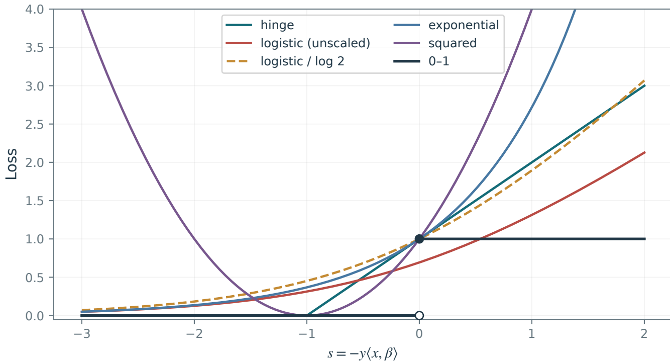
Classification losses versus negative margin
